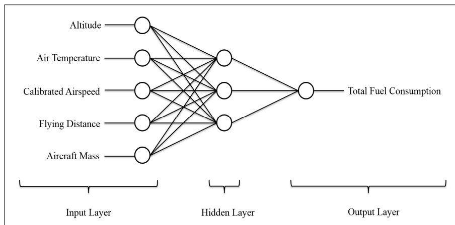
Fig. 2. Fuel consumption estimation model for terminal airspace redesigns
