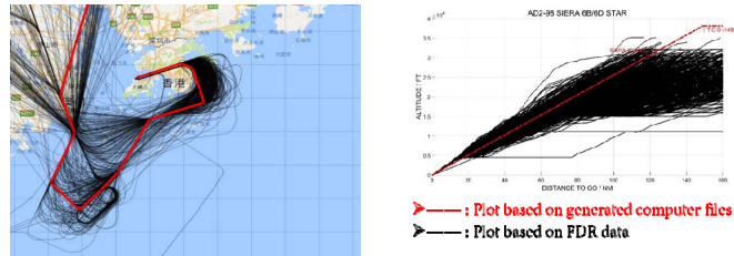
(c) Horizontal & vertical plot for SIERA-6B/6D
