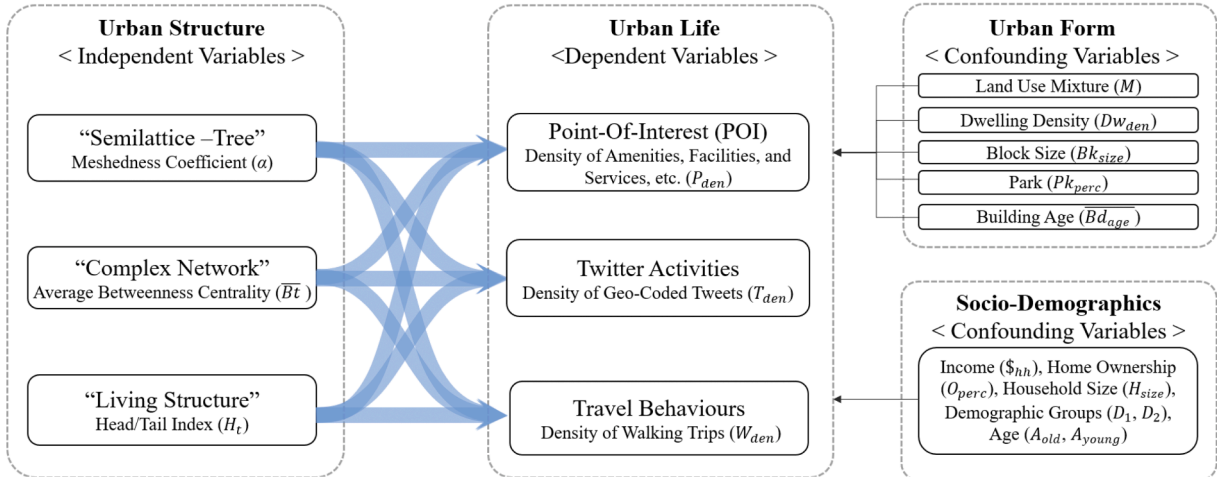
Fig. 2. A conceptual framework for testing Alexander's theory on urban structure and urban life.
