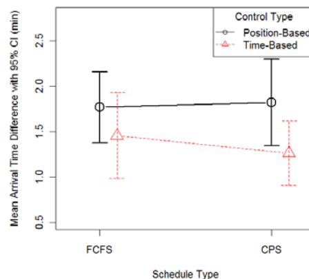
Figure 9. Schedule Conformance
