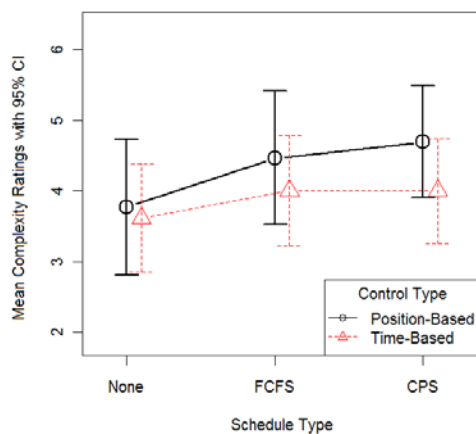
Figure 11. Perceived Complexity
